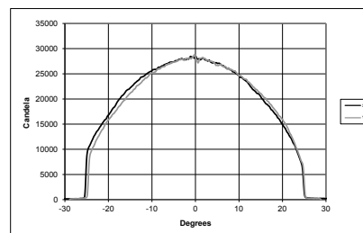
Candela Plot
